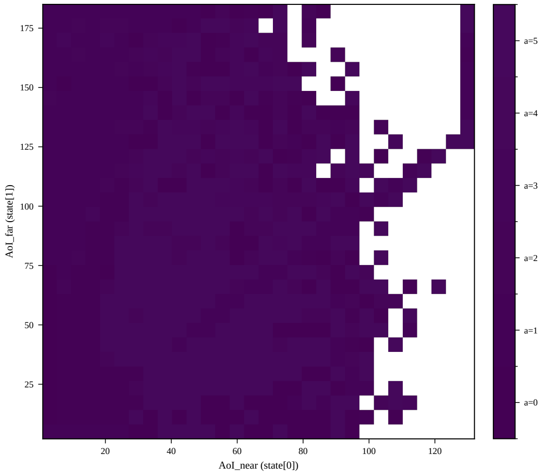
Most Likely Action (AoI_near vs AoI_far)
